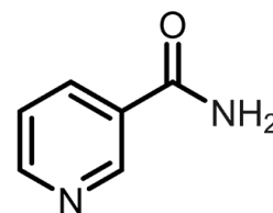
Nicotinamide (niacinamide)
